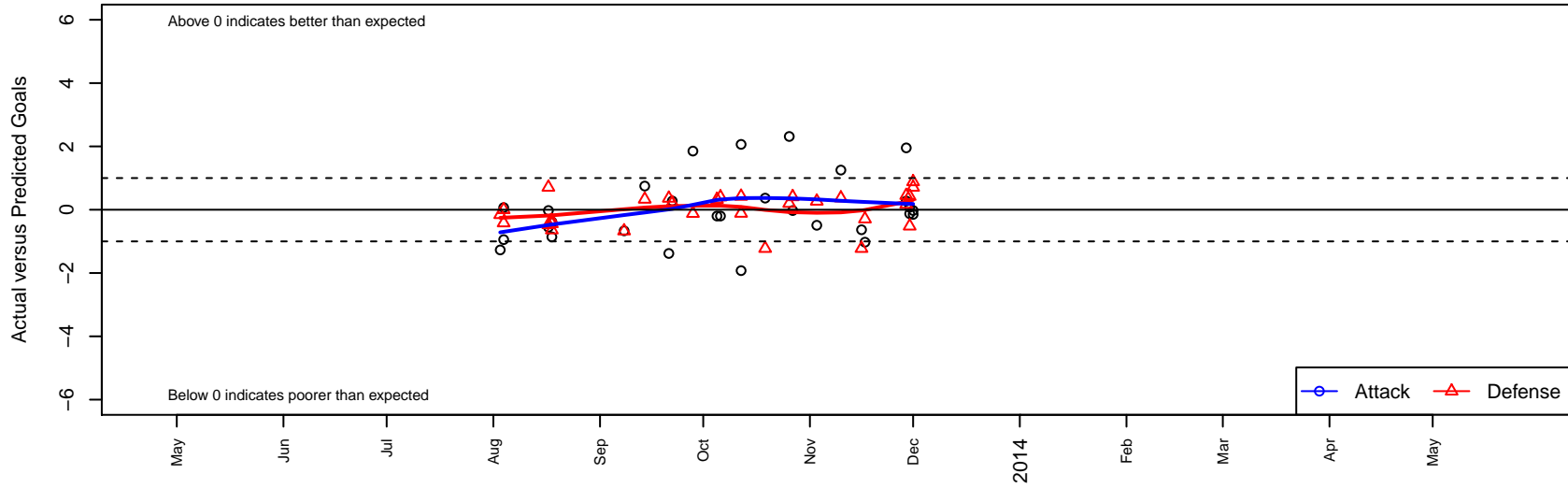
Legends FC G00 Dots are actual minus expected GF (blue circles) and GA (red triangles). Blue line is smoothed change in attack strength. Red is smoothed change in defense strength.
